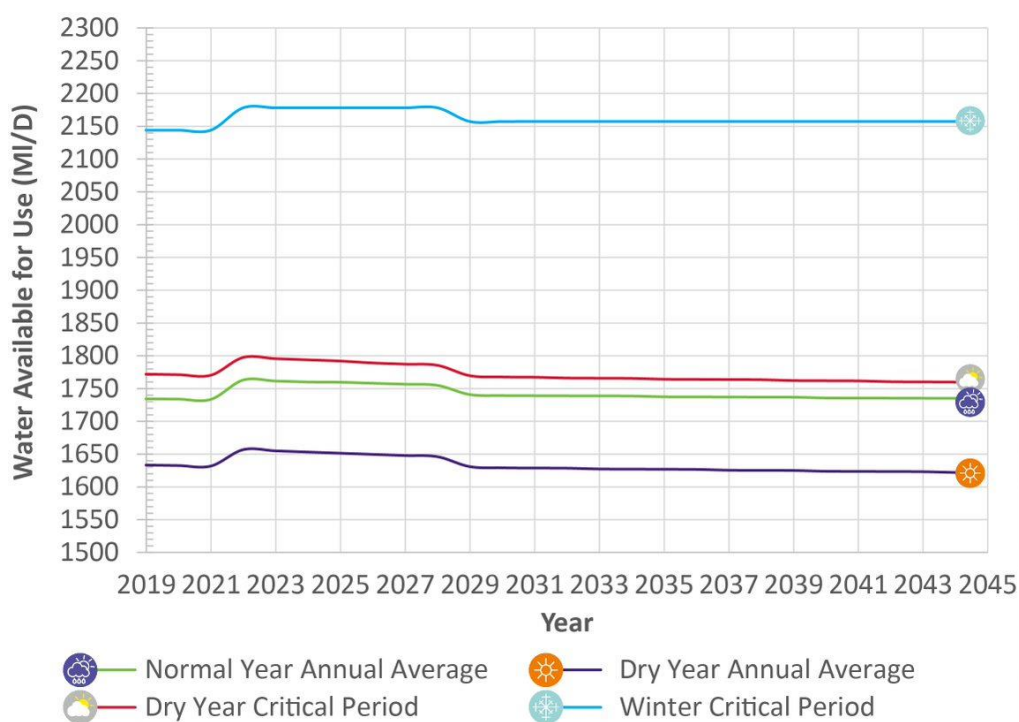
Figure 3.8 – National Summary of WAFU, 2019 to 2044
