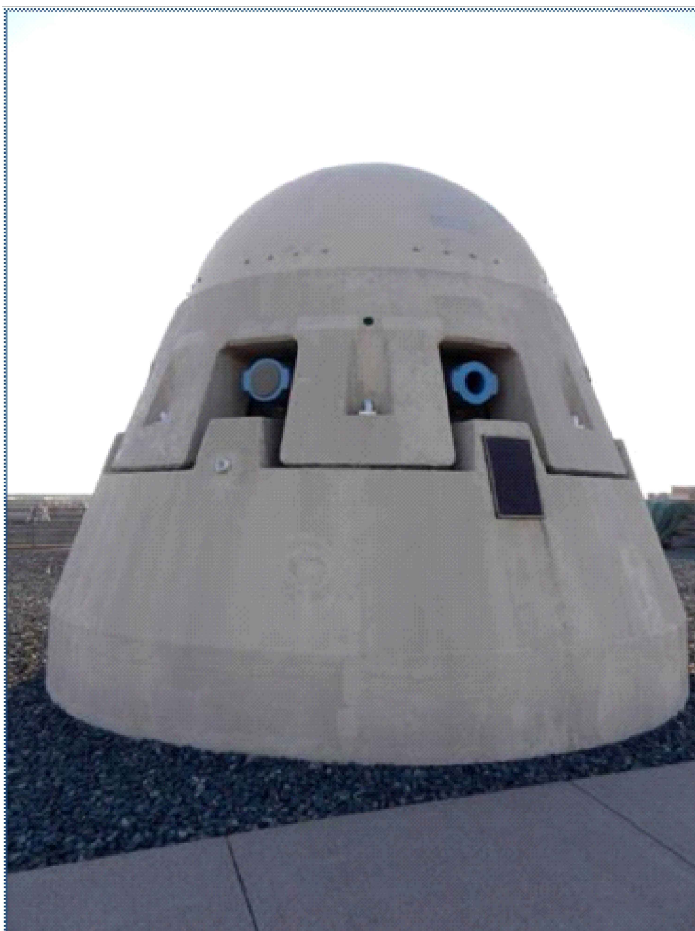
TYPICAL MARINE RISER & DIFFUSER SYSTEM
