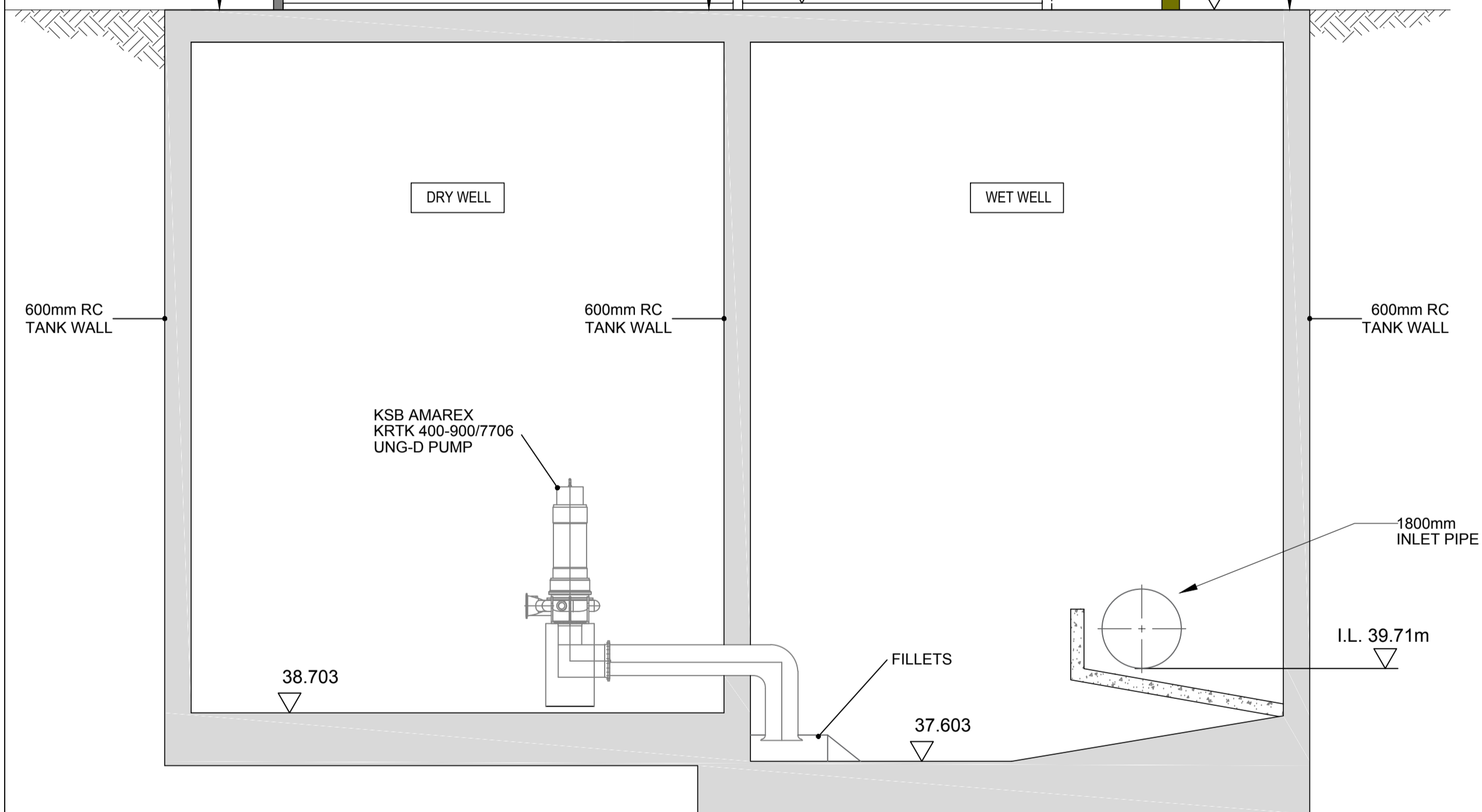
1 SECTION SCALE 1:100
