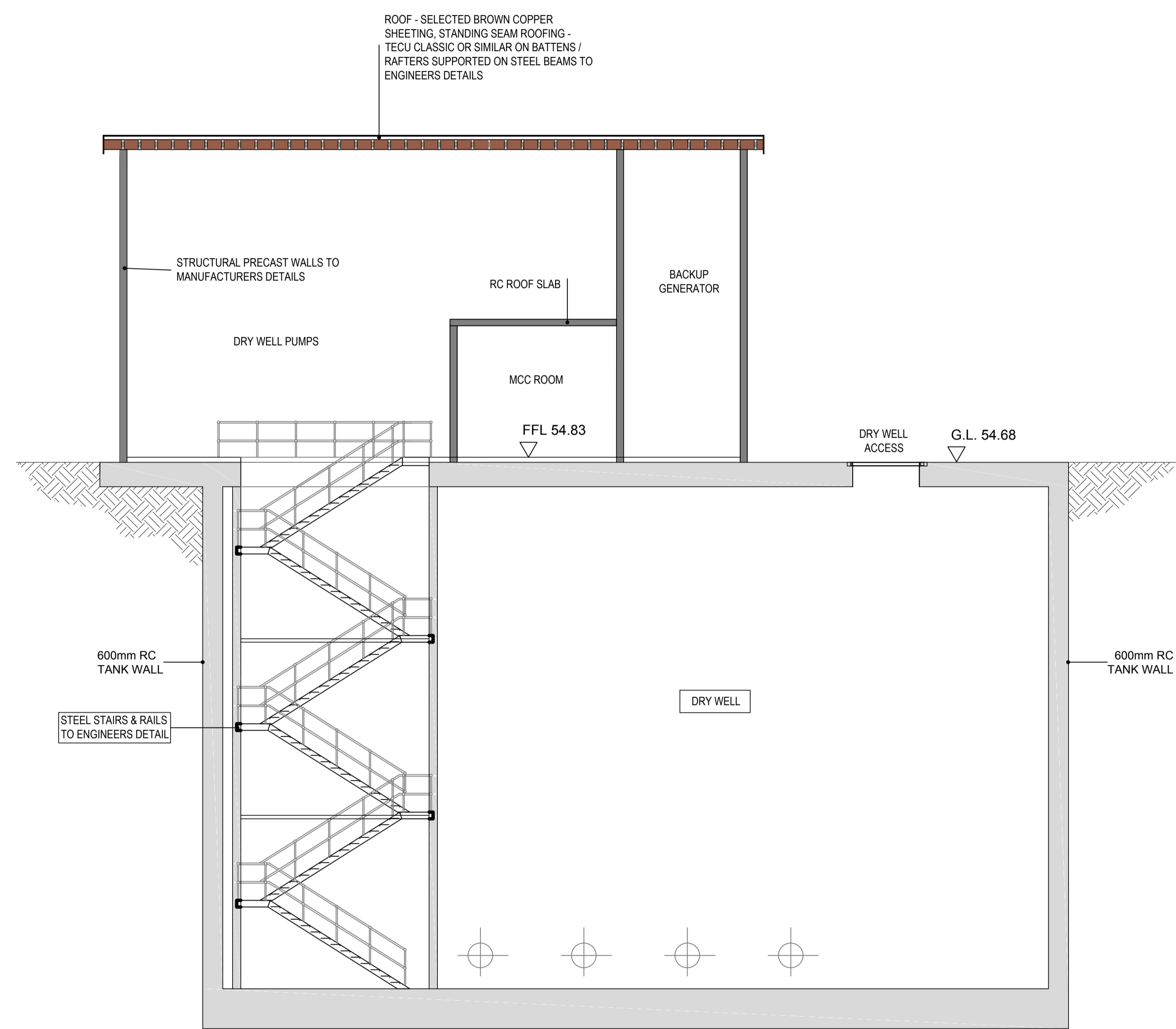
2 SECTION SCALE 1:100
