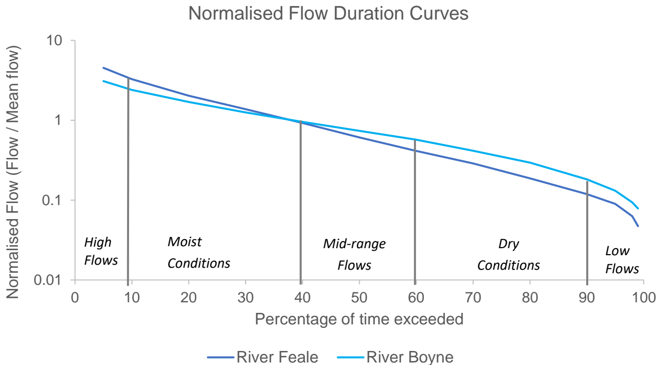
Figure 3.9 Hydrological Characteristics of the River Feale and River Boyne
